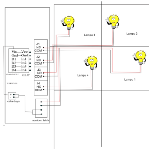
Gambar 3 Perancangan Hardware
