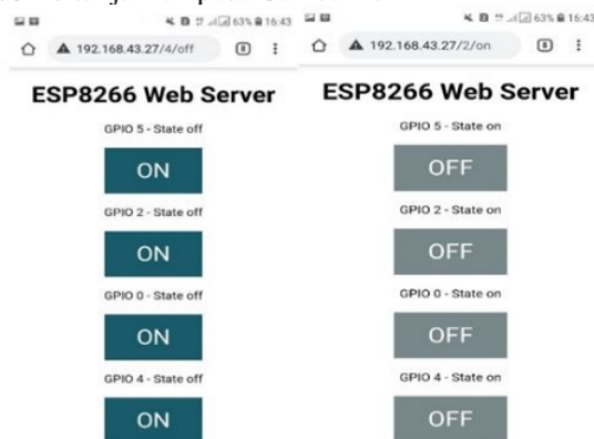
Gambar 4 Tampilan Kendali Tombol On/Off
